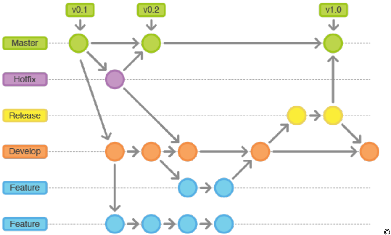
Seibert - Git-Workflows: Der Gitflow-Workflow
