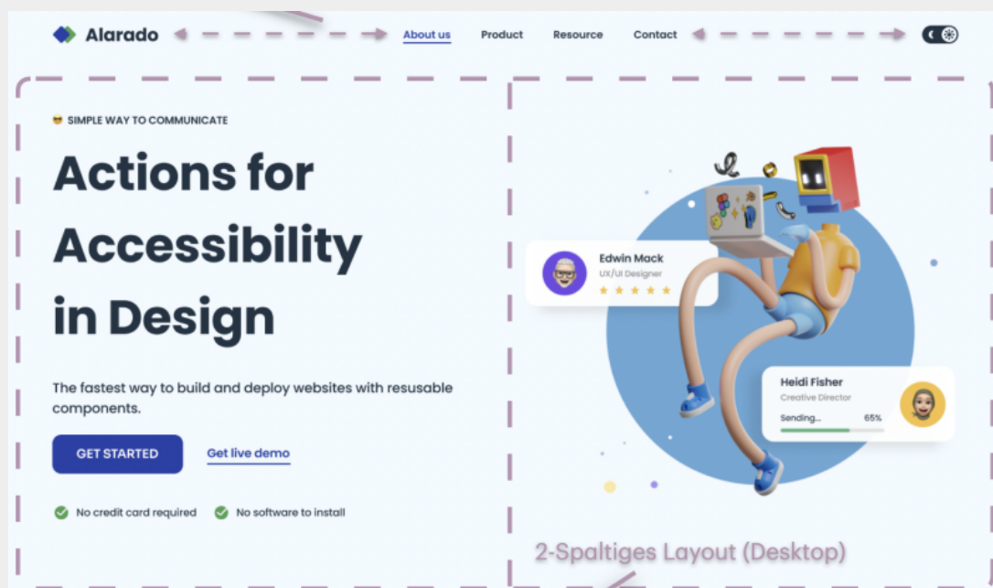
Flexbox-Layout
