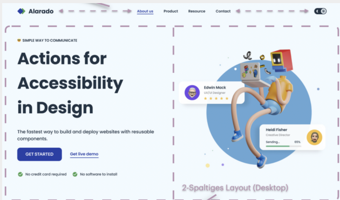
Flexbox-Layout
