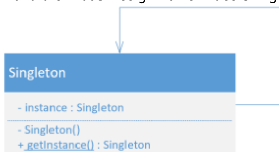
//Abb. 6.13: //Singleton-Pattern
